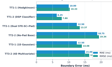
Overall VAD Boundary Error Benchmark (4 Test Recordings)
